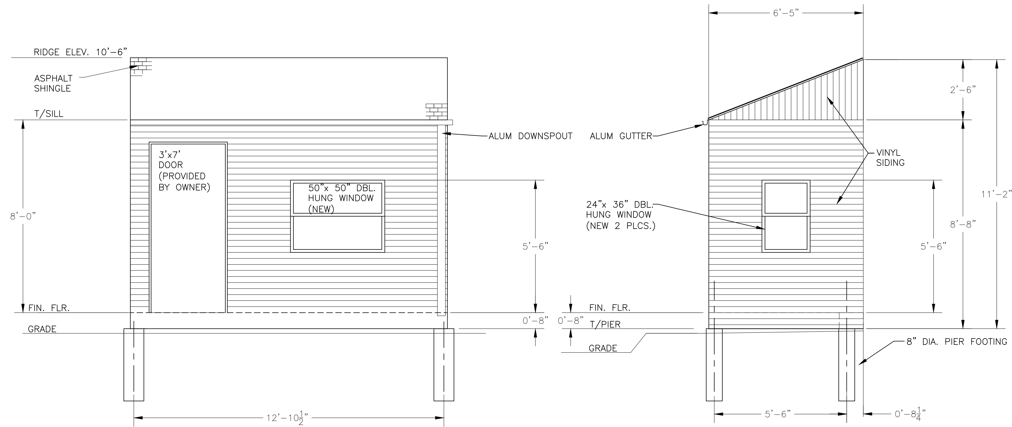
FRONT VIEW
