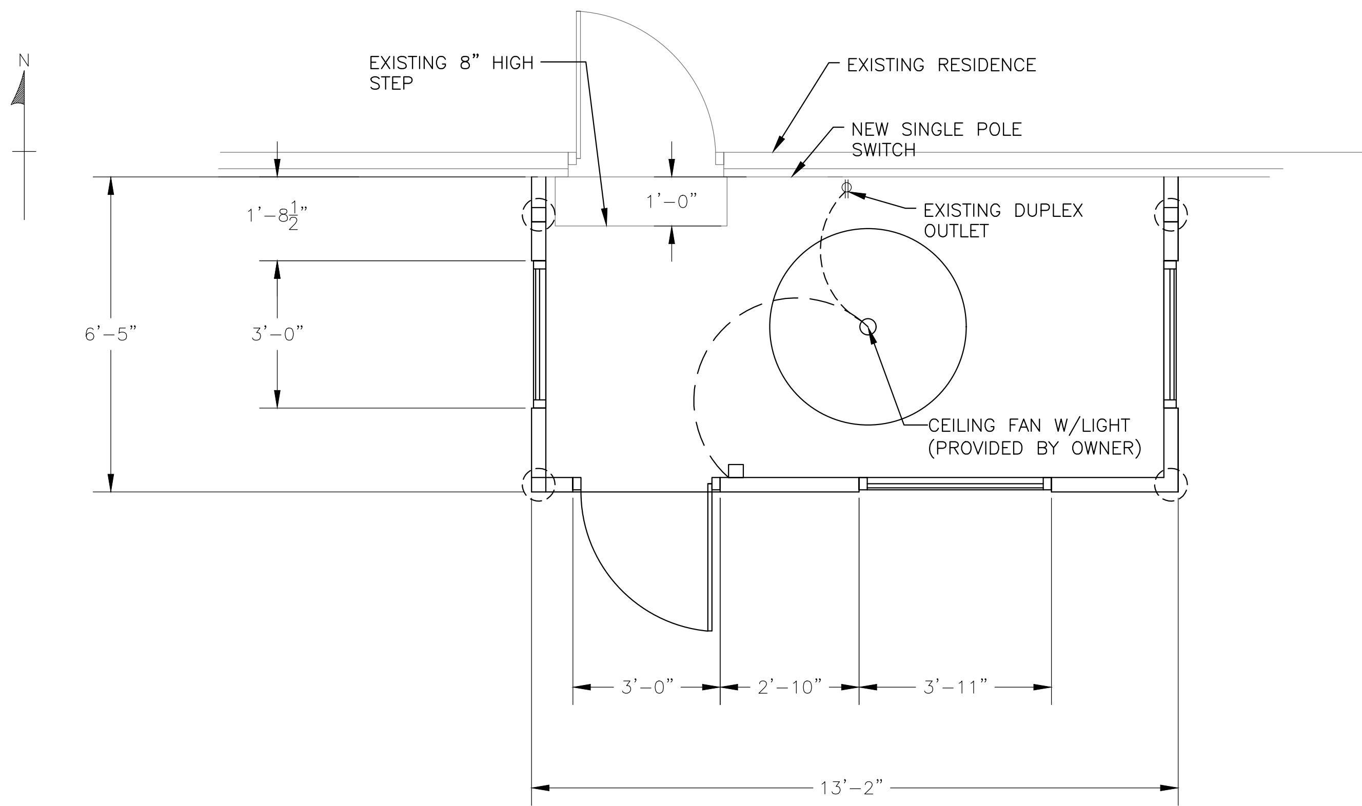
PLAN VIEW
